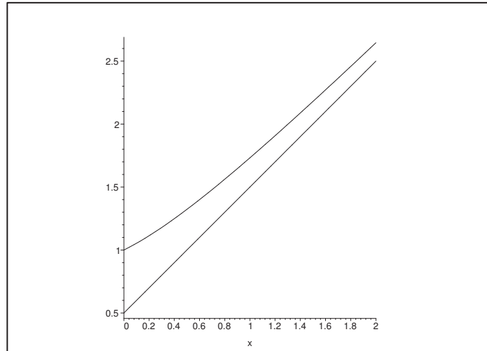
Figure 38: The function y = \sqrt{x^2 + x + 1} and its asymptote y = x + \frac{1}{2} .
