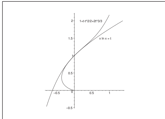
Figure 41: The graphs of x \cdot \ln x = t and x = 1 + t - \frac{1}{2}t^2 + \frac{2}{3}t^3 . Notice that the graph of the implicit given function bends back towards the Y -axis, so it cannot be described as a function in t in the whole range where it is defined.
