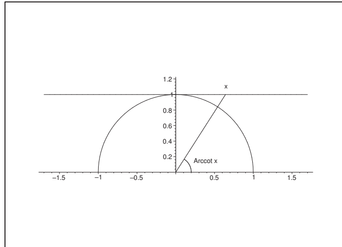
Figure 22: If x is the coordinate on the axis through (0, 1) parallel with the X -axis, then \operatorname{Arccot} x is the angle between the positive X -axis and the vector (x, 1) .
