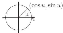
Figure 42: The unit circle and the trigonometric functions.
